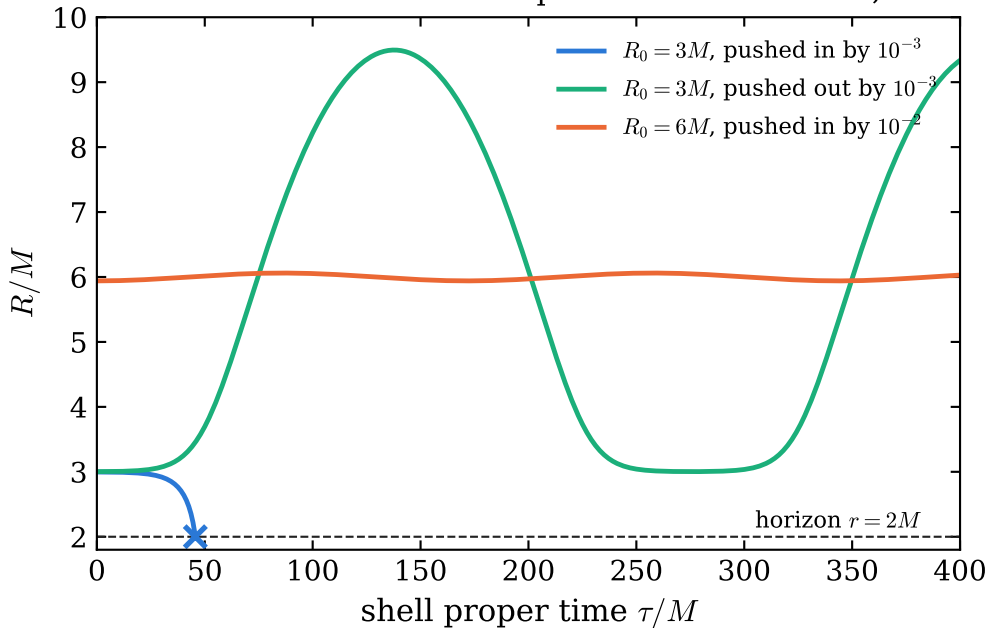
Nonlinear radial evolution of perturbed static shells, \Gamma = 2
